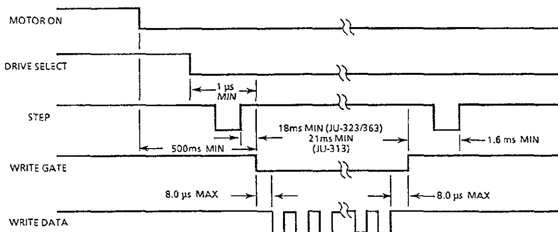
FIGURE 1-8 WRITE INITIATE TIMING
