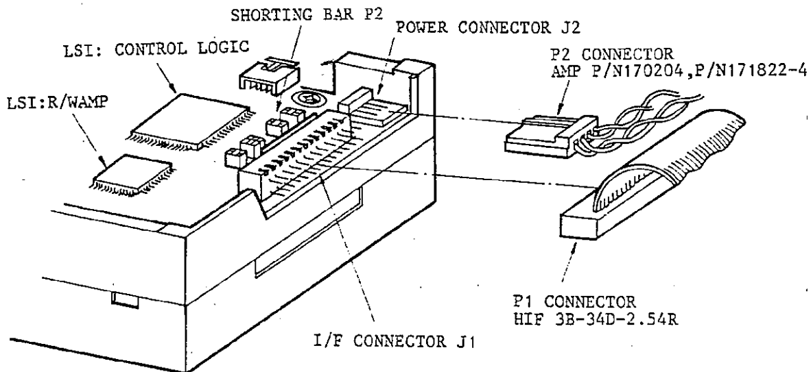
FIGURE 3-1 INTERFACE CONNECTORS LOCATIONS
