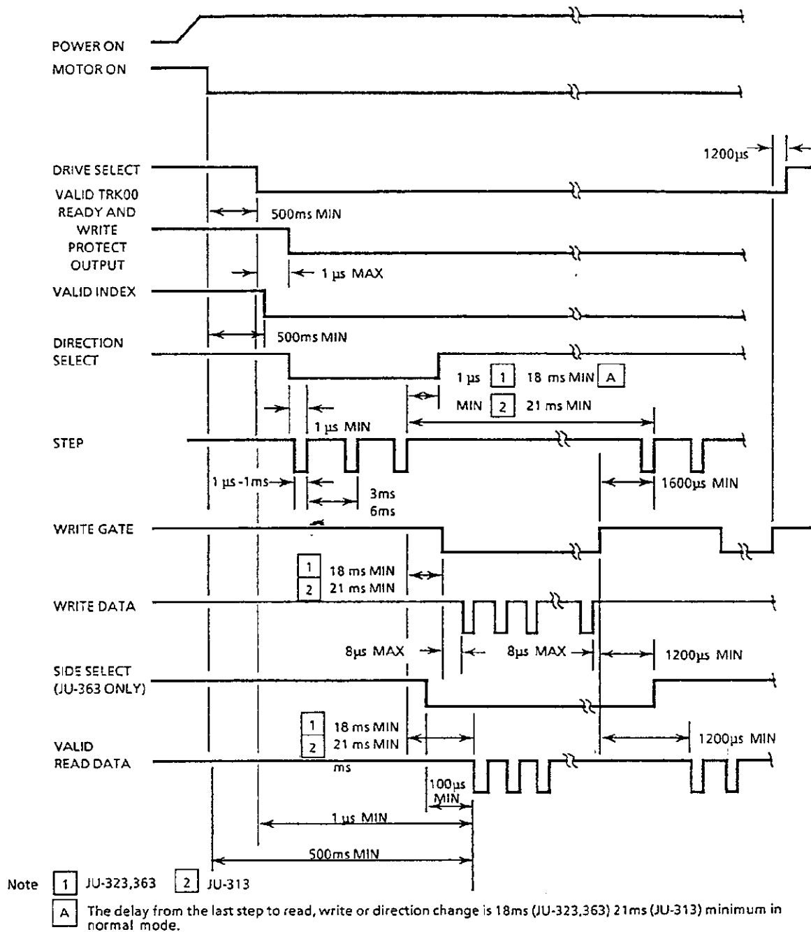
FIGURE 1-10 GENERAL CONTROL AND DATA TIMING REQUIREMENT
