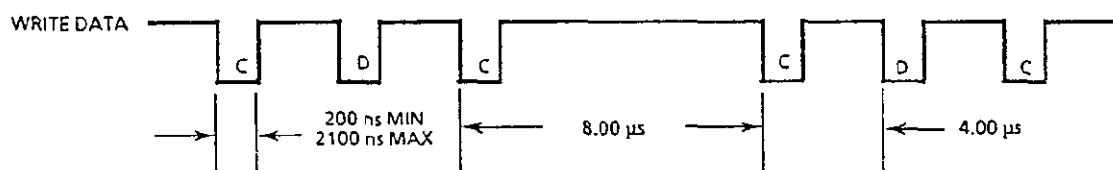
FIGURE 1-9 WRITE DATA TIMING (FM)
