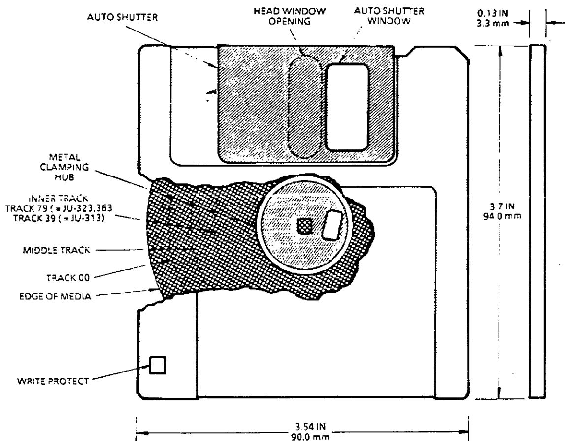
FIGURE 8-2 MICROCARTRIDGE NOMENCLATURE
