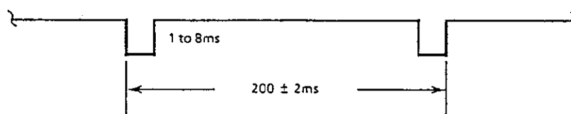
FIGURE 2-4 INDEX TIMING
