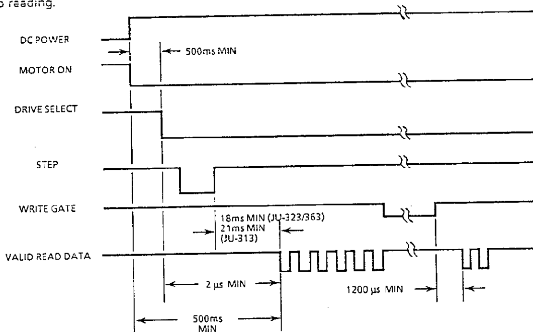
FIGURE 1-5 READ INITIATE TIMING
