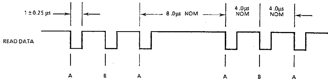
FIGURE 1-6 READ DATA TIMING (FM)
