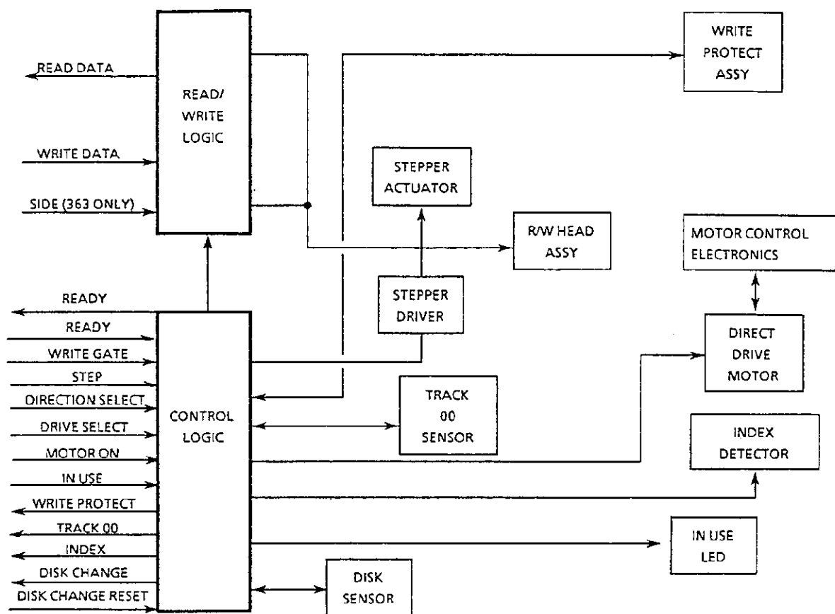
FIGURE 1-2 JU3X3 FUNCTIONAL DIAGRAM
