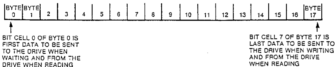
FIGURE 6-2. DATA BYTES
