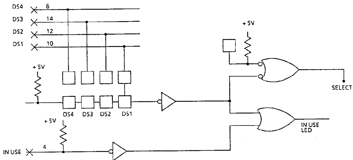
FIGURE 7-1 DRIVE SELECT LOGIC
