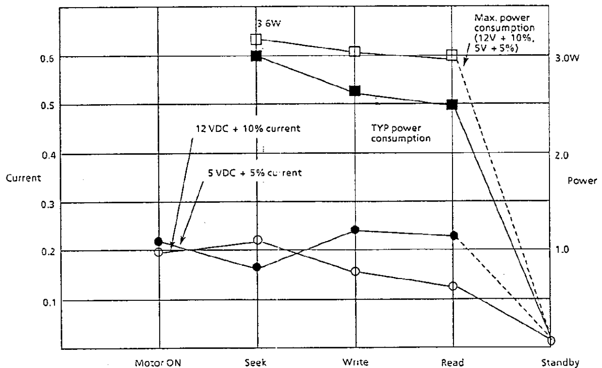
FIGURE 1-1 CALCULATION METHOD OF POWER CONSUMPTION
