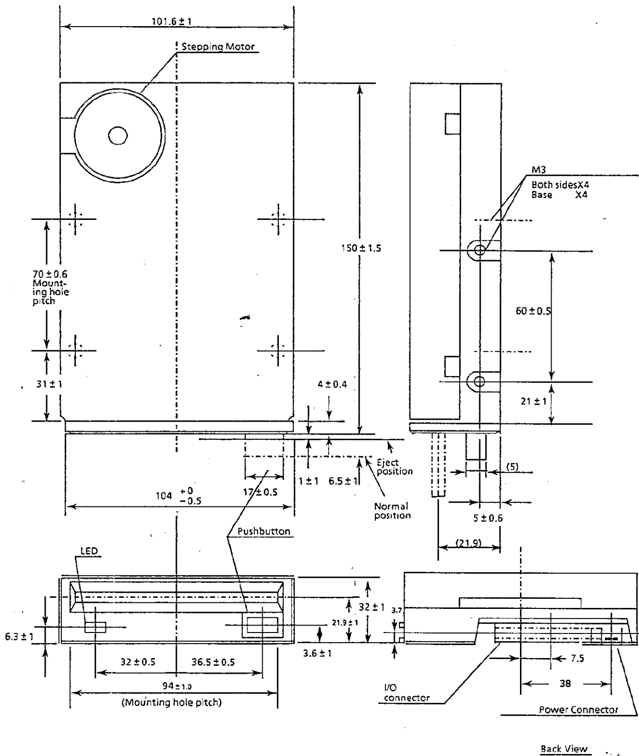
FIGURE 4-2. MECHANICAL DIMENSIONS
