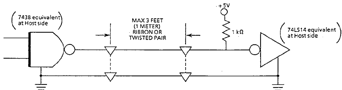
FIGURE 2-2 INTERFACE SIGNAL DRIVER/RECEIVER
