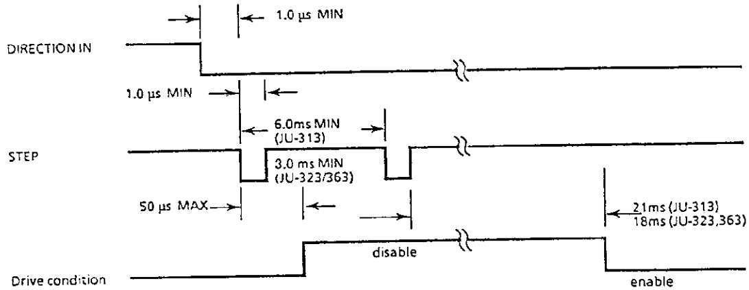
FIGURE 1-4 NORMAL STEP MODE
