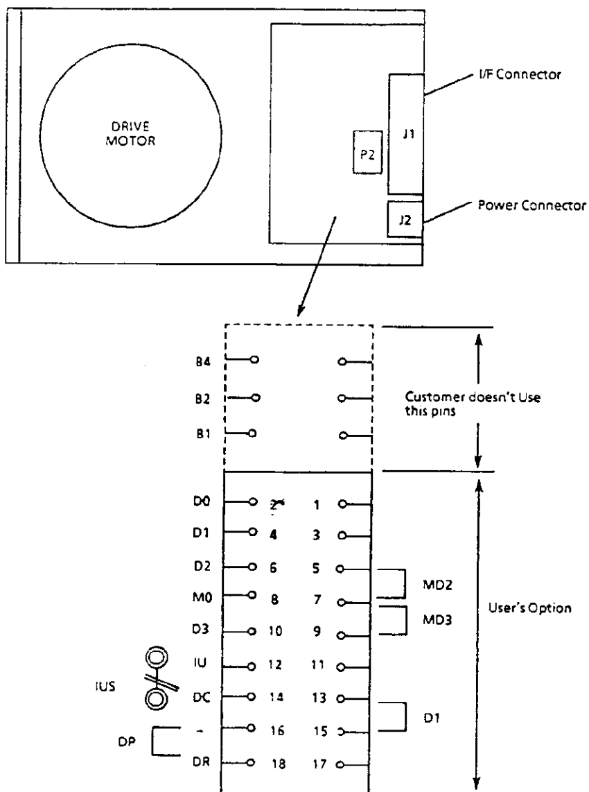
FIGURE 7-2 SHORTING BAR P2 PIN ASSIGNMENT
