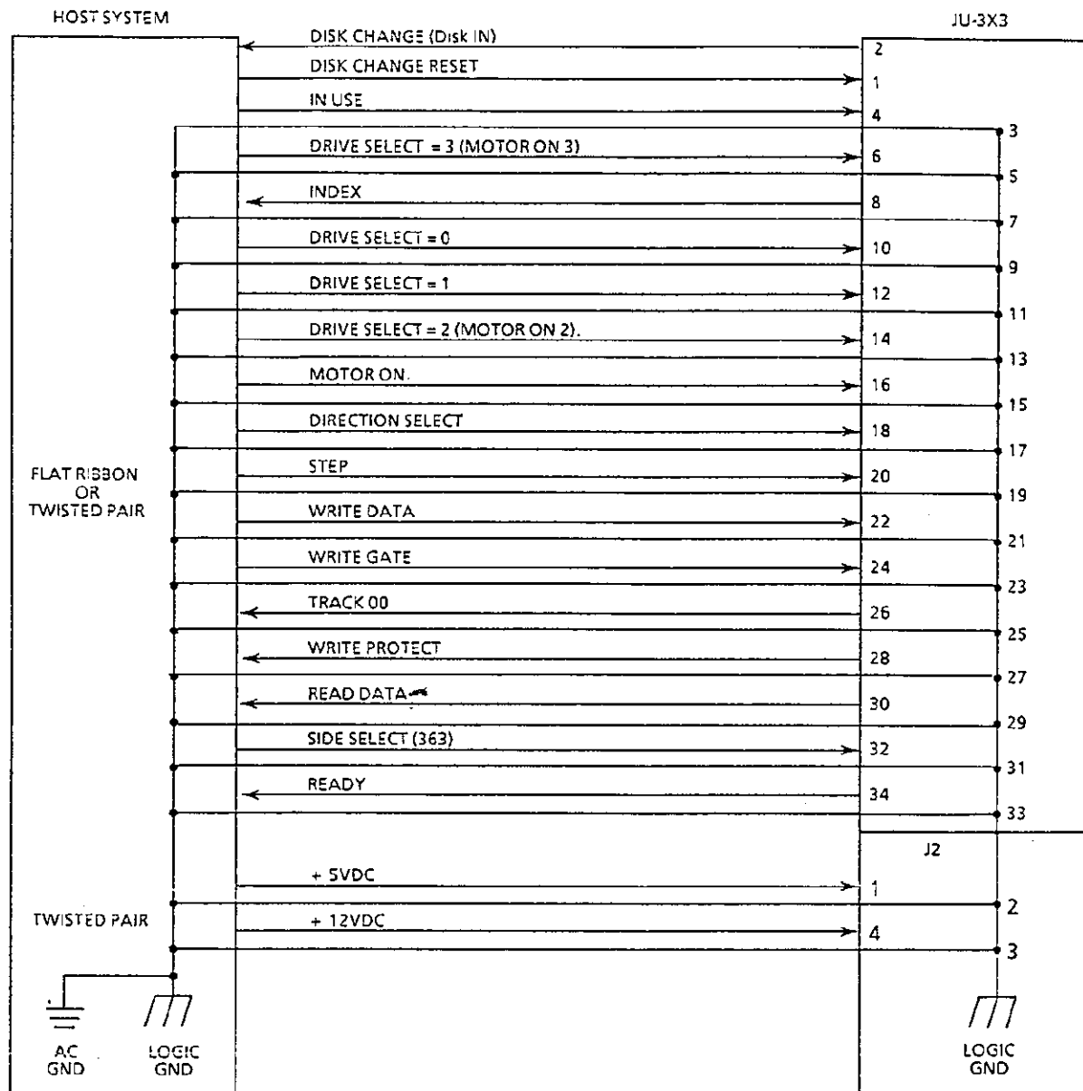
FIGURE 2-1 INTERFACE CONNECTIONS
