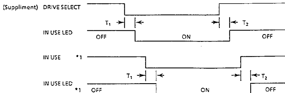
FIGURE 1-10 GENERAL CONTROL AND DATA TIMING REQUIREMENT
